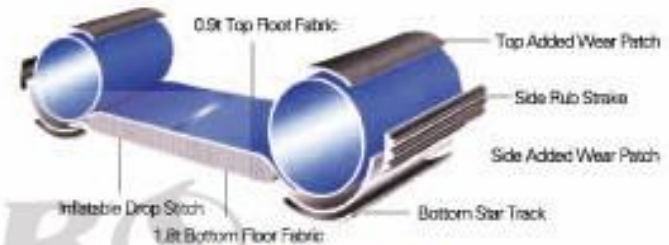
Floor Construction(DS)
